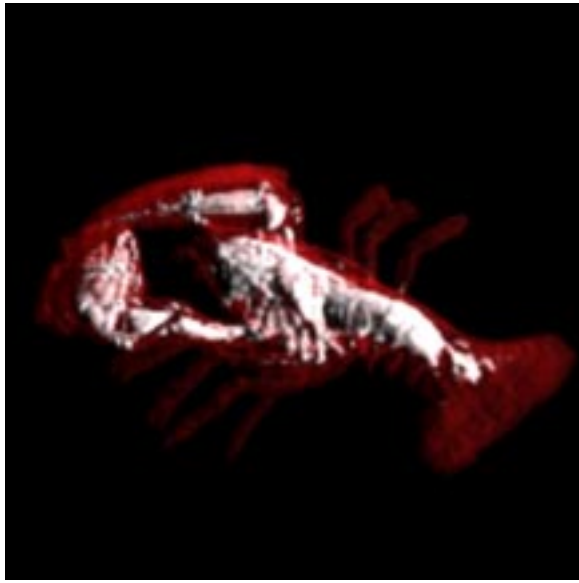
Figure 5: CT scanned Lobster dataset with a translucent shell rendered in 0.26 seconds at 200^2 resolution
